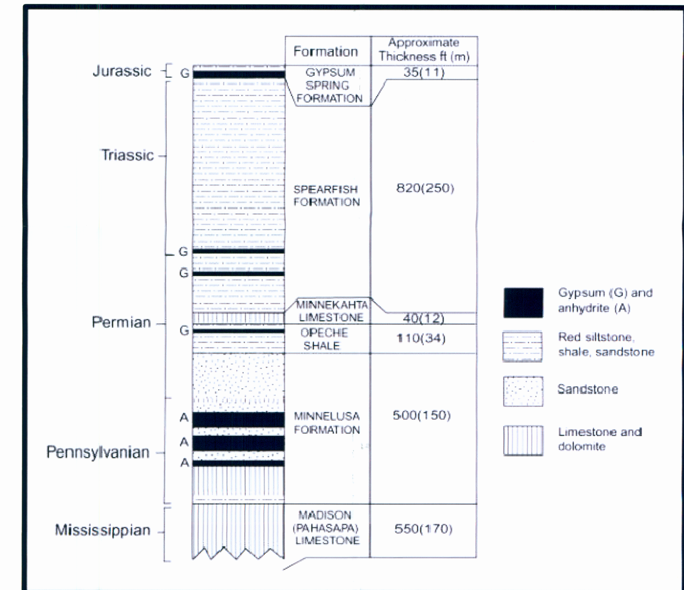
STRATIGRAPHIC SECTION of the BLACK HILLS FIGURE 2 NOT TO SCALE
