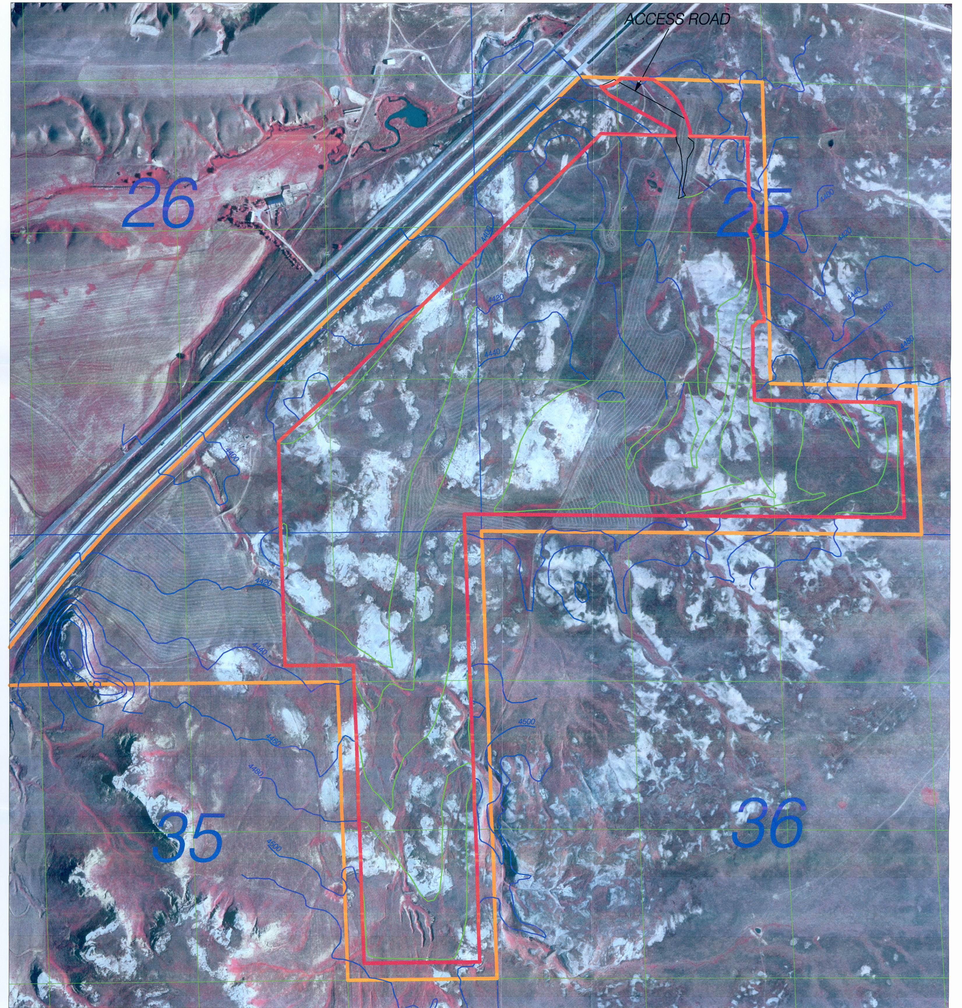
PLAN VIEW MAP WITH POST MINE TOPOGRAPHY Scale 1" = 500 Feet
