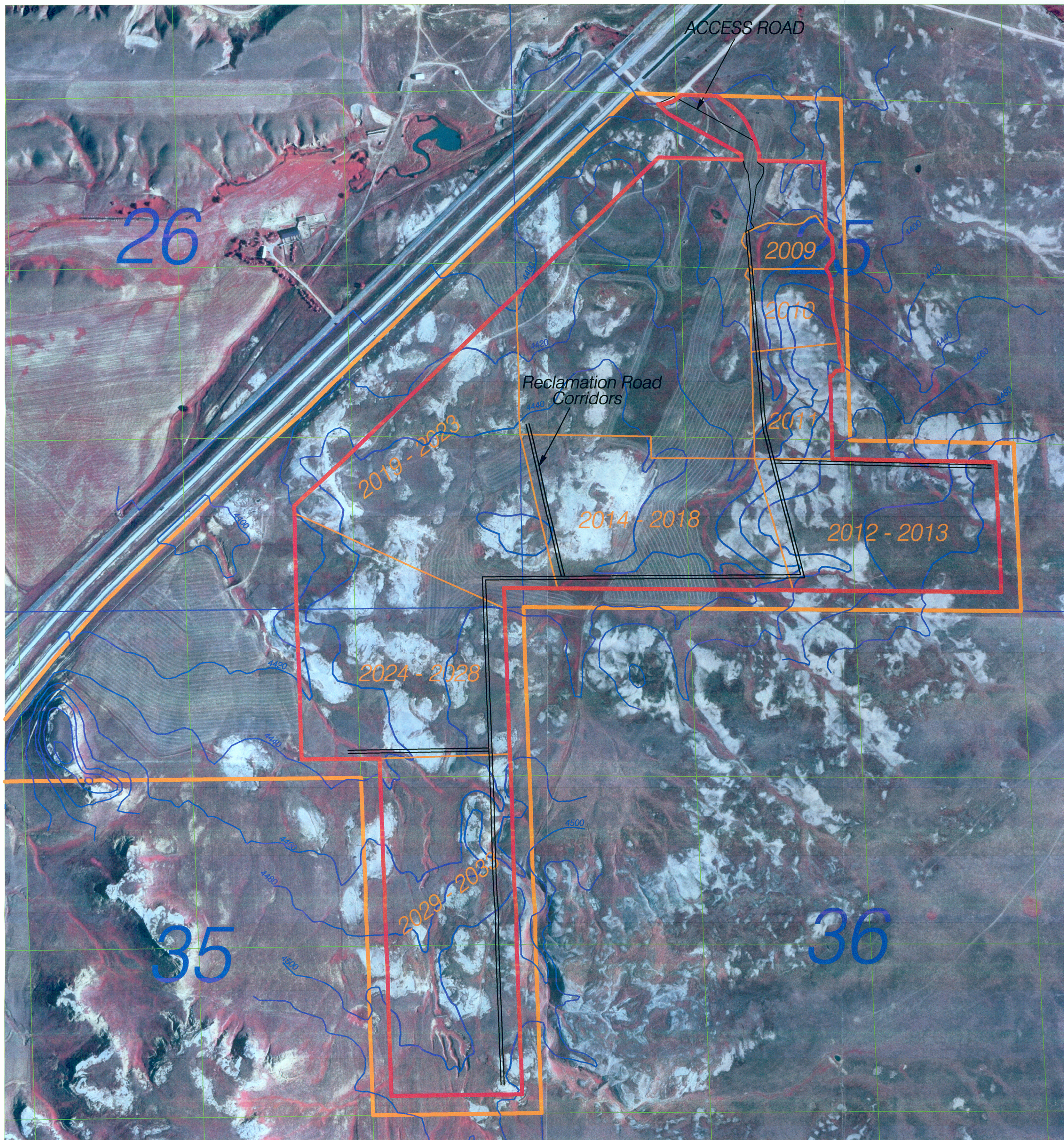
PLAN VIEW MAP WITH RECLAMATION PROGRESSIONS AND PREMINE TOPOGRAPHY Scale 1" = 500 Feet
