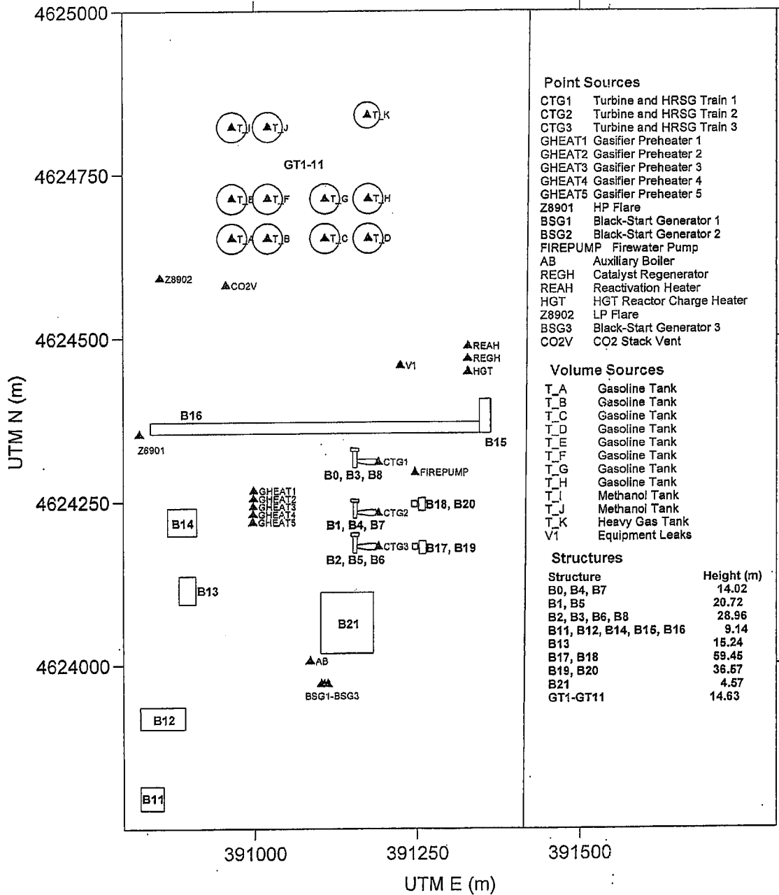
Figure 4 – Point and Volume Sources, Structures for Proposed IGL Plant
