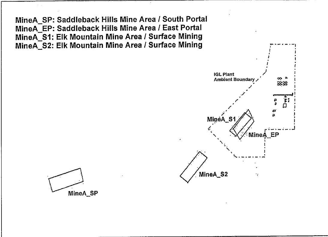
Figure 5 – Area Source Locations
