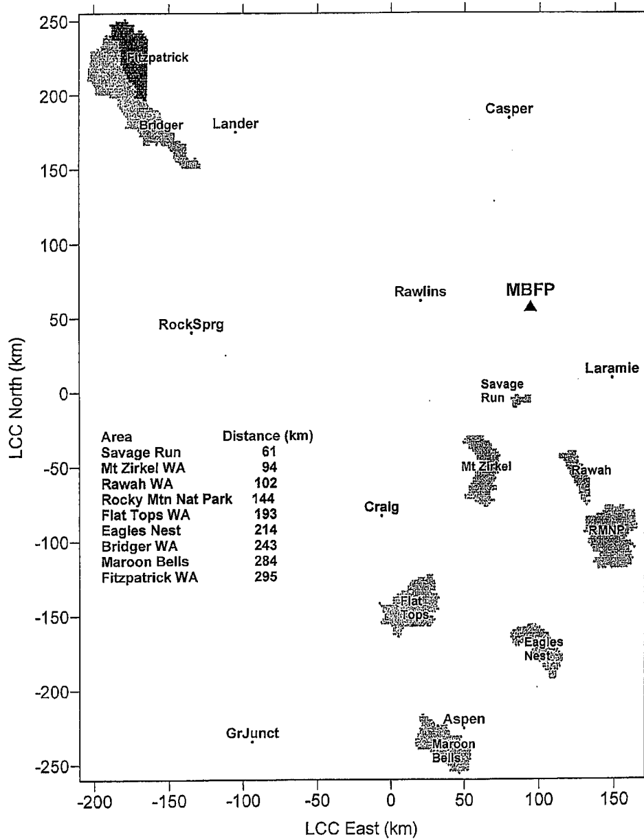
Figure 11 – Location of Proposed Project vs. Class I Areas
