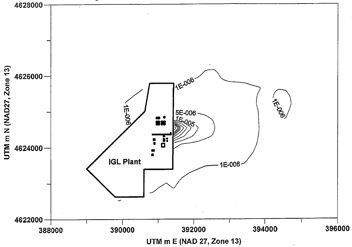
Figure 10 - Modeled Increased Cancer Risk for Benzene
