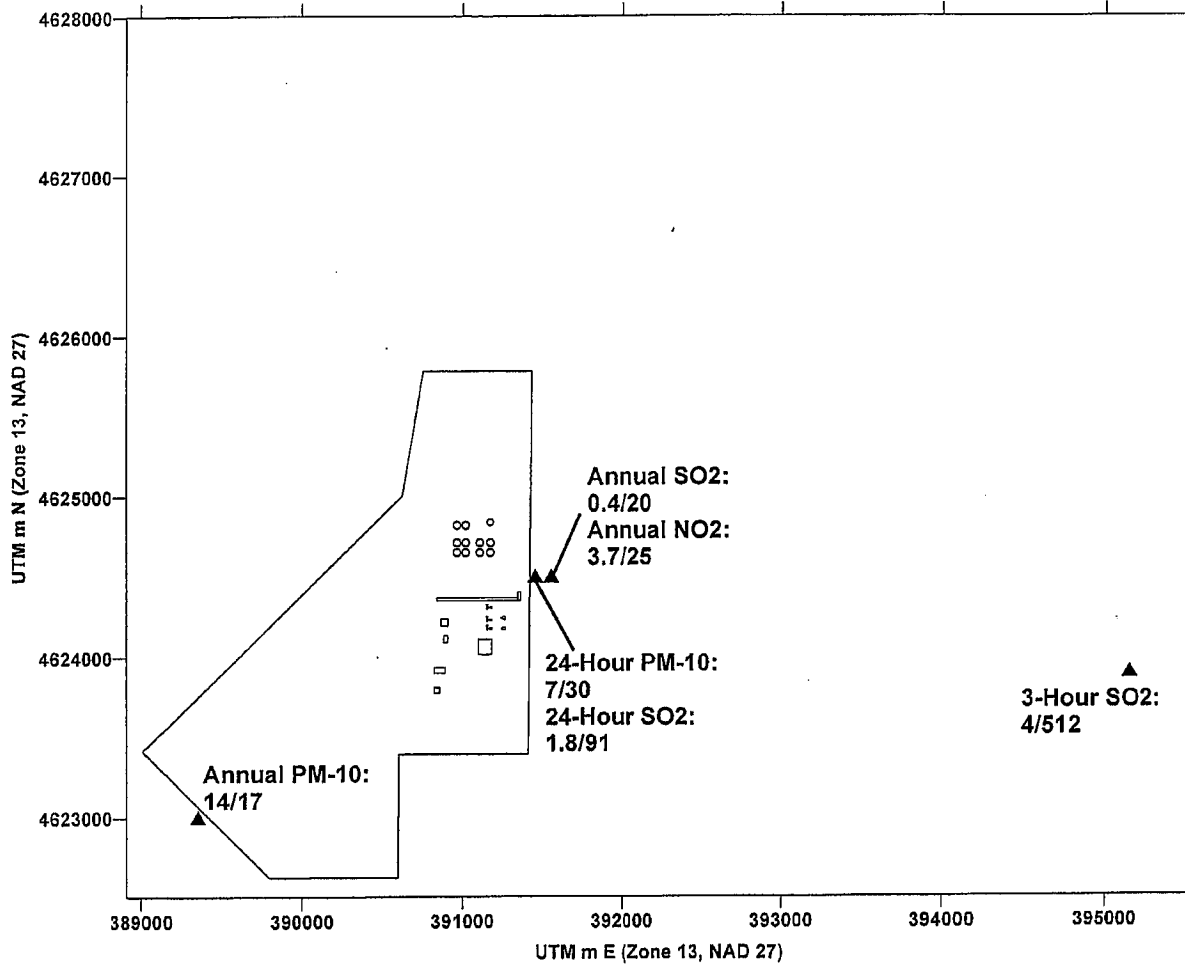
Figure 8 - Locations of Modeled Maximums (PSD Increments)
