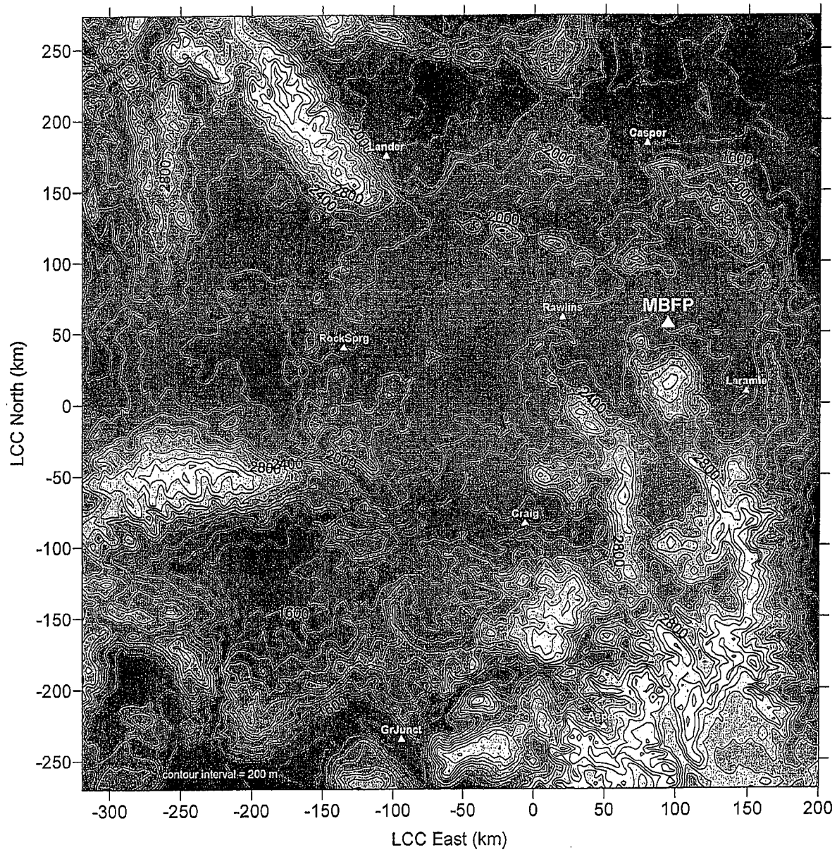
Figure 13 – Terrain for the CALMET/CALPUFF Domain
