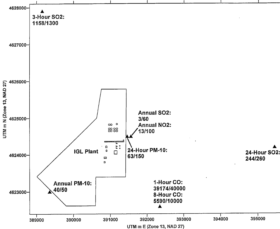
Figure 7 - Locations of Modeled Maximums (WAAQS/NAAQS)
