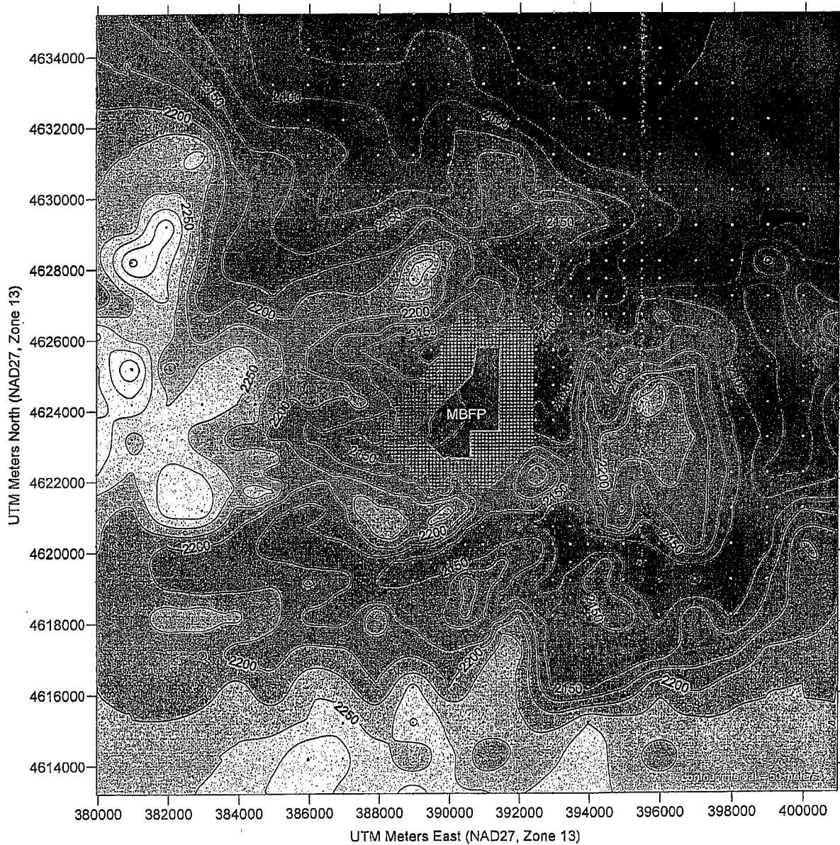
Figure 3 – Base AERMOD Receptor Grid
