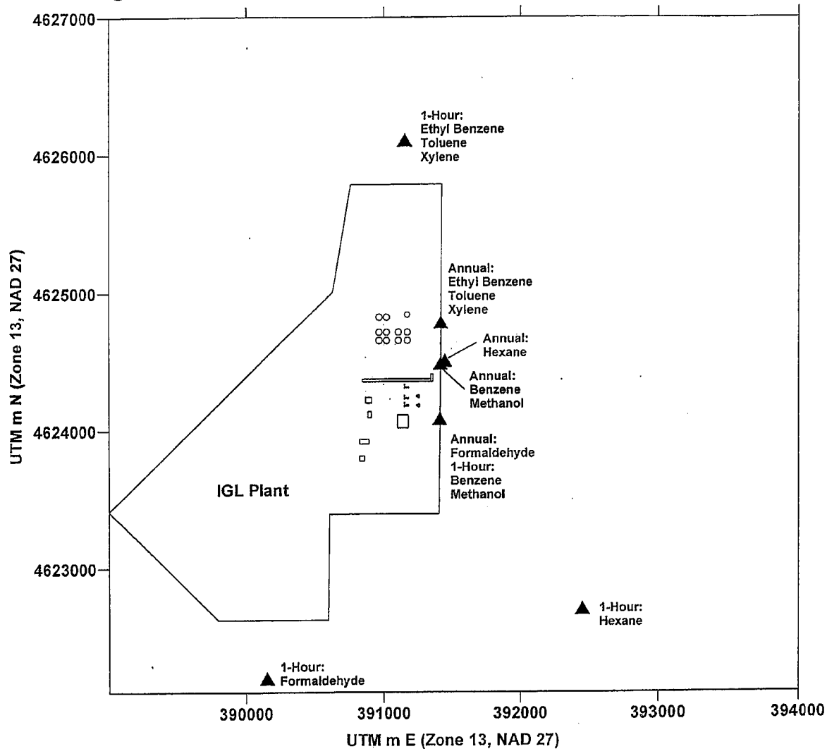
Figure 9 - Locations of Modeled Maximum 1-Hour or Annual HAP Exposures
