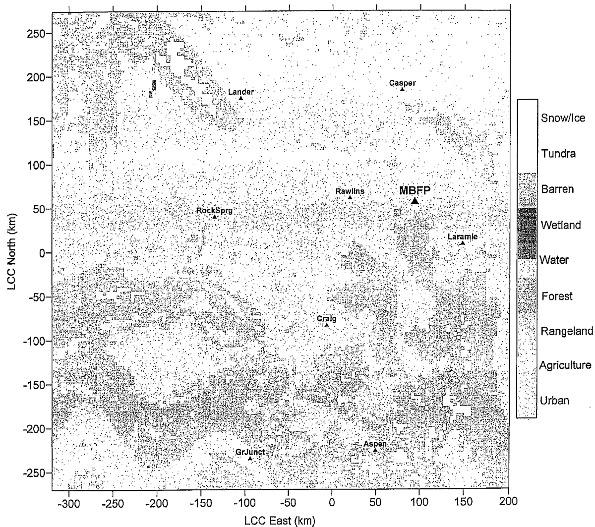
Figure 12 – Land Use for CALMET/CALPUFF Domain
