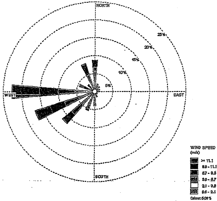
Laramie Field CALMET-predicted Windrose (grid cell:118, 71)-743 hours
