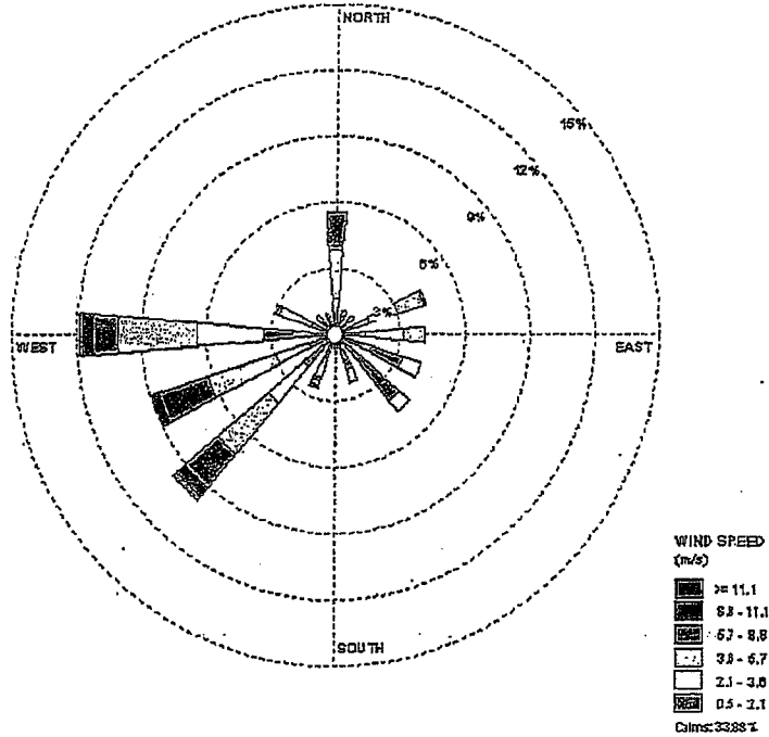
Figure 15 - Laramie field Windroses (March, 2003)
