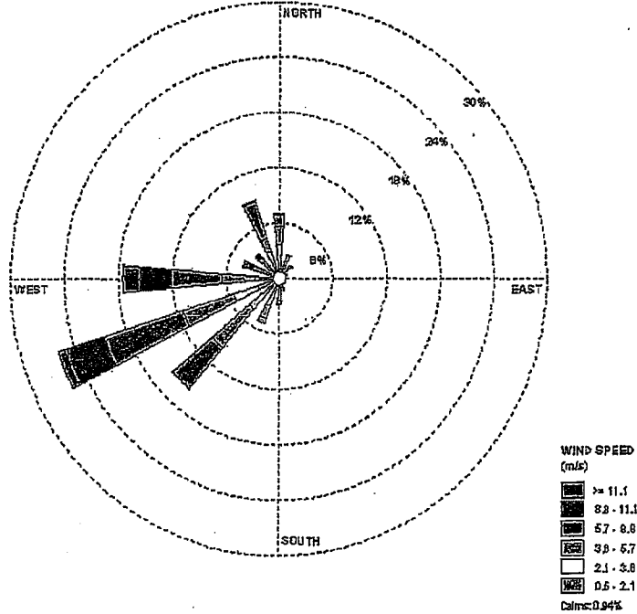
Laramie Field CALMET-predicted Windrose (grid cell:118, 71)-743 hours
