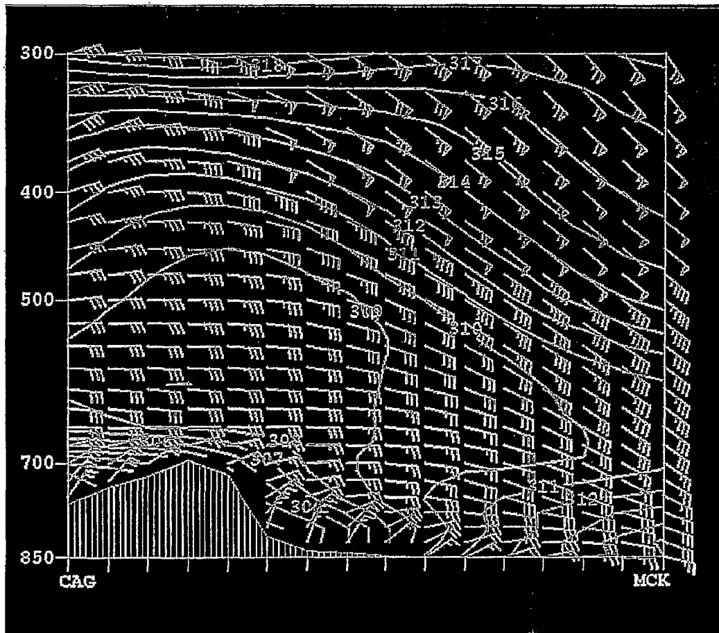
Fig. 3 Vertical cross section showing equlv. potential temp. (K) and winds (knots), 6-hr. forecast from the Eta model initialized at 18 UTC 18 Mar.
