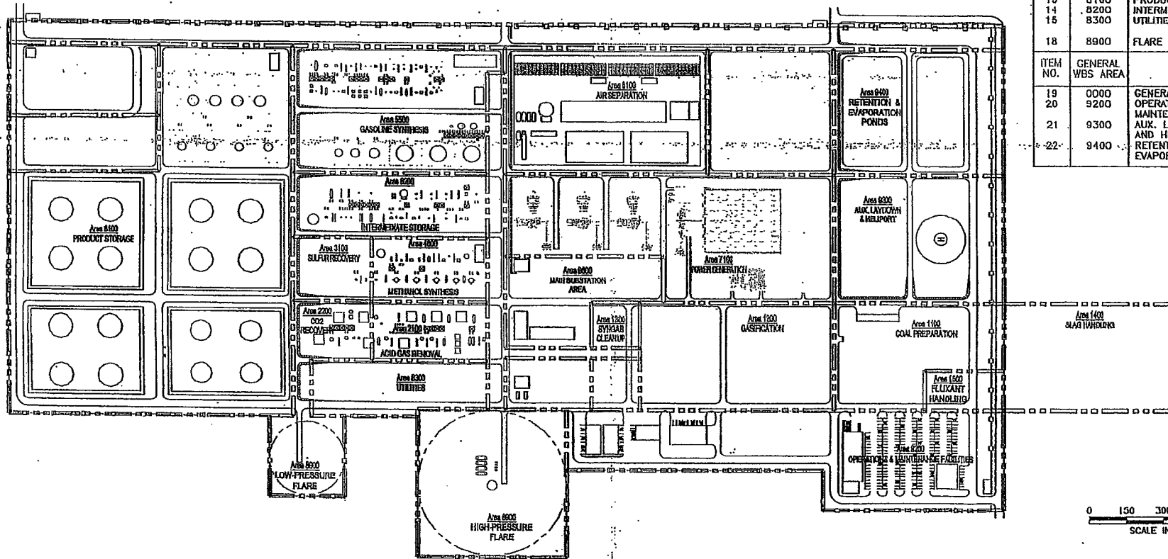
FIGURE 1.4 MEDICINE BOW FUEL & POWER PROCESS EQUIPMENT LAYOUT DRAWING INDEX / WBS INDEX
