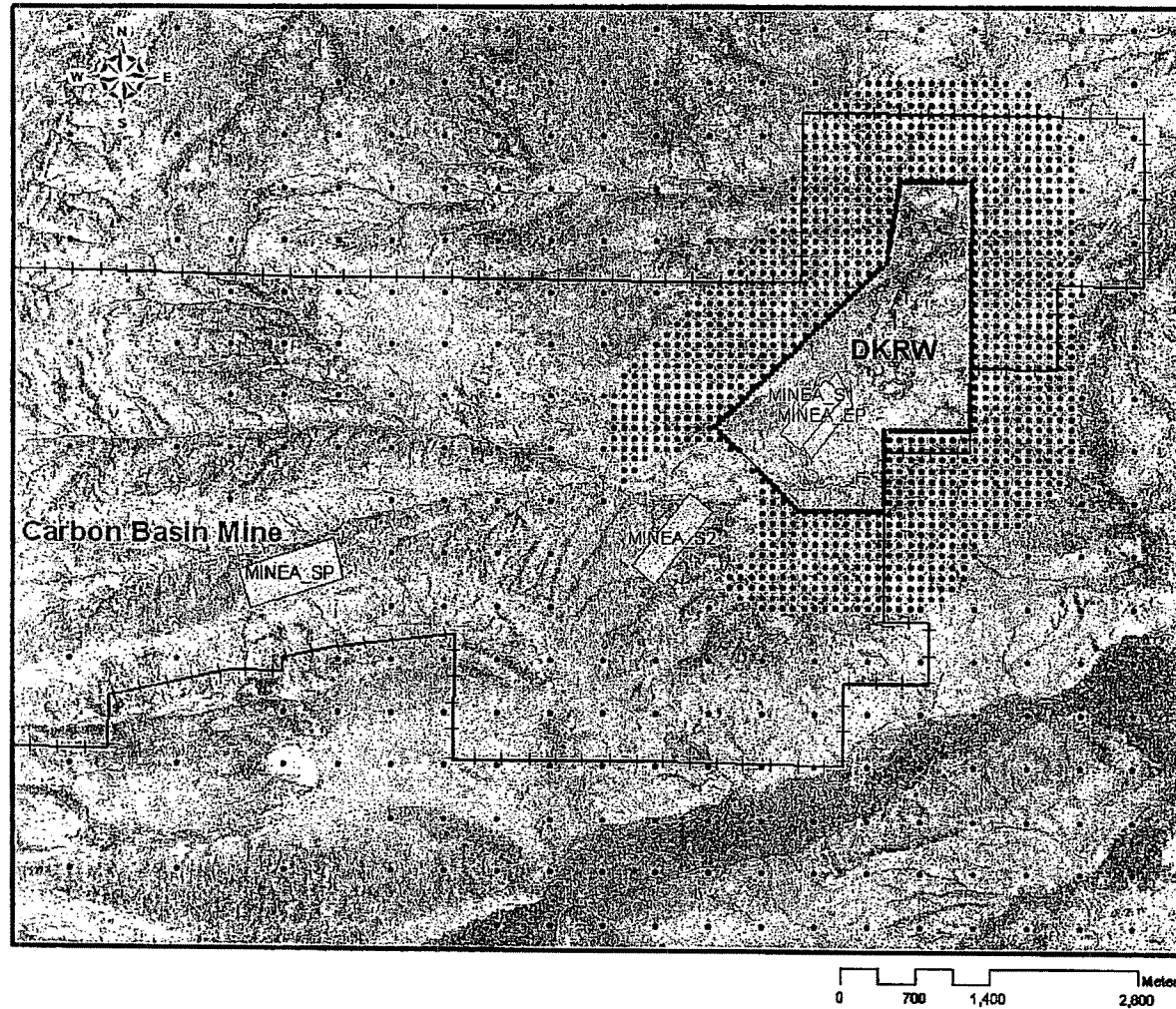
Figure 3: Mine Area Sources and Model Receptors
