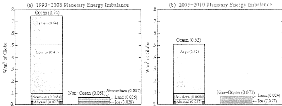
Figure 3. (a) Estimated planetary energy imbalance in 1993-2008, and (b) in 2005-2010. Data sources are given by Hansen et al. (2011).
