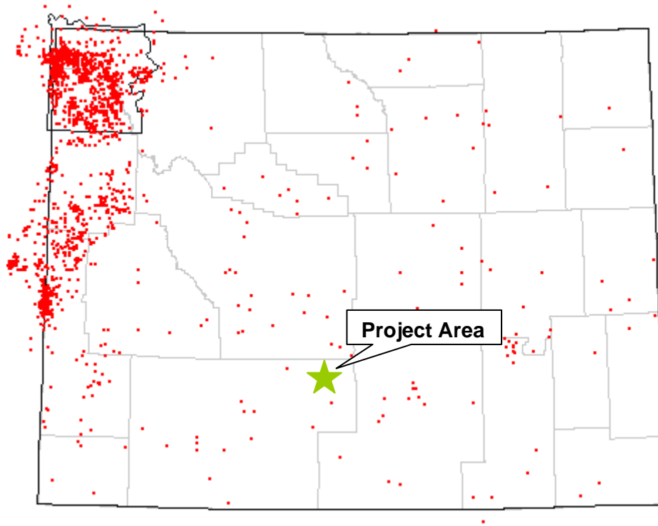
Figure D5-3 Historical seismic activities in Wyoming*
