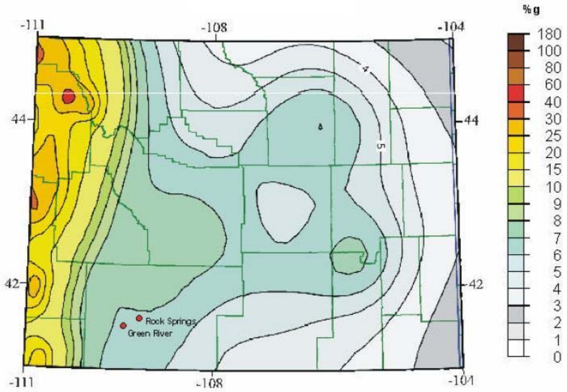
Figure D5-6. 500-YEAR PROBABLISTIC ACCELERATION MAP OF WYOMING (Case et. al., 2002)
