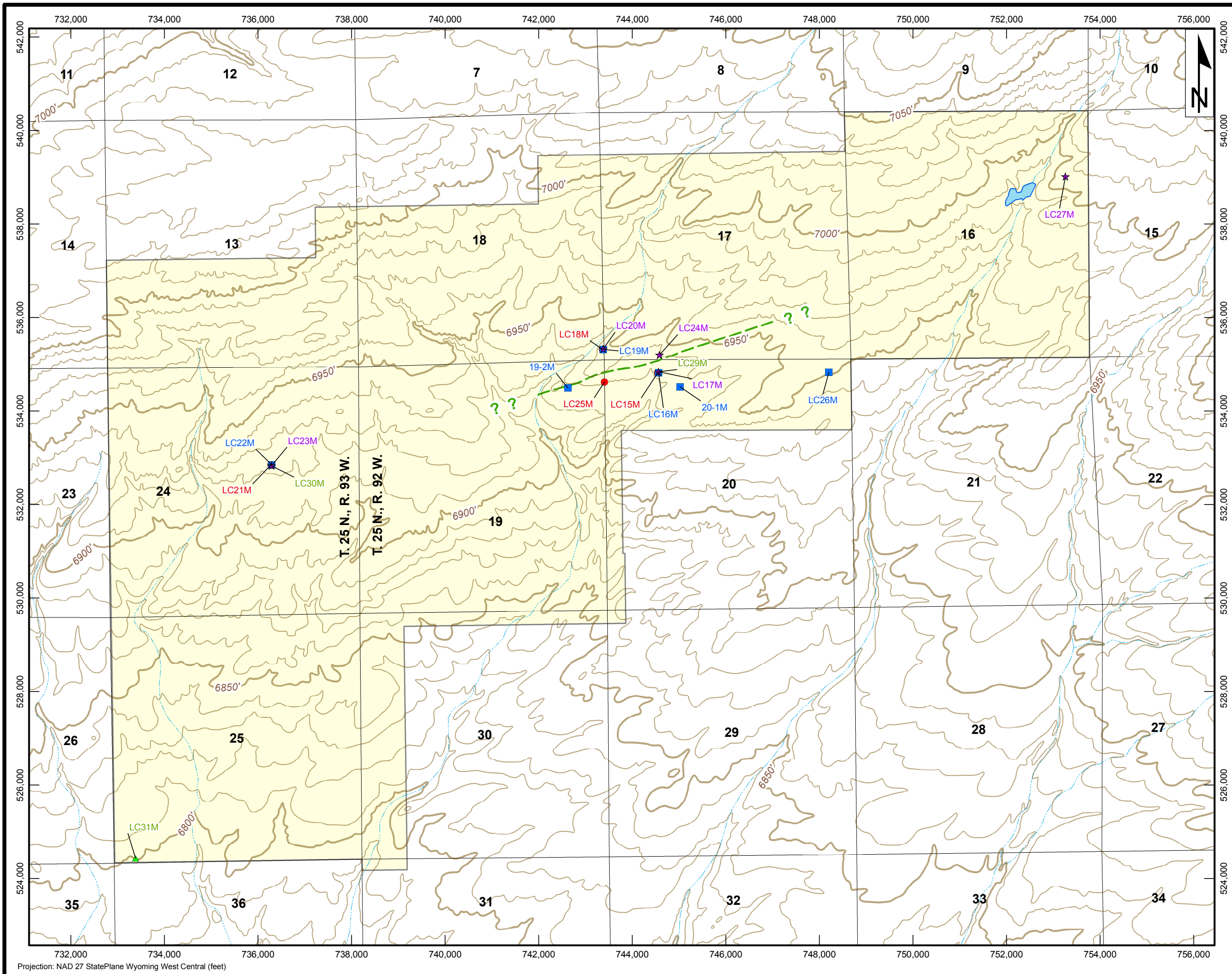
FIGURE D6-13 Location of Pump Tests Conducted in 1982 and 2006 Lost Creek Permit Area
