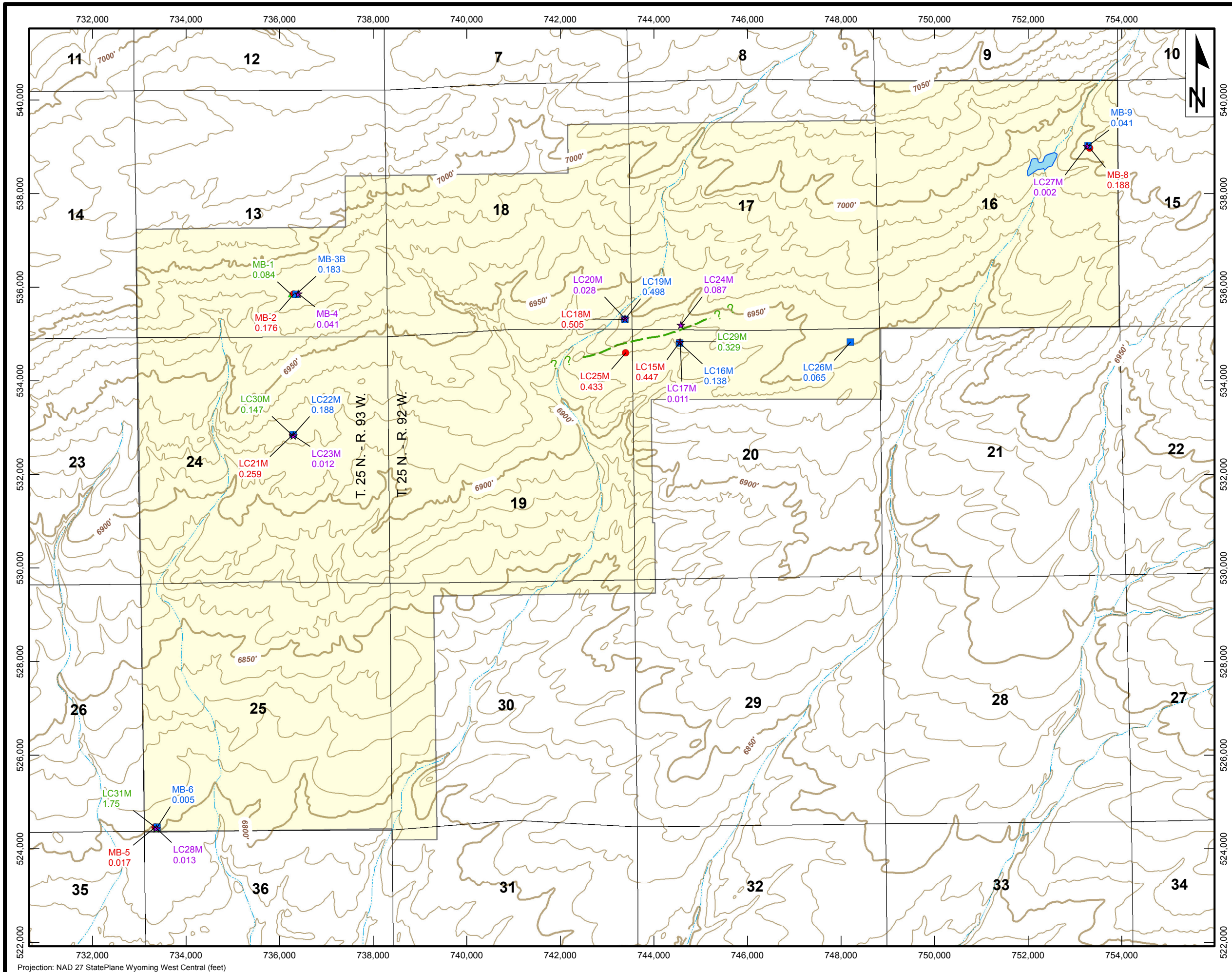
FIGURE D6-28a Distribution of Average Uranium September 2006 to July 2010
