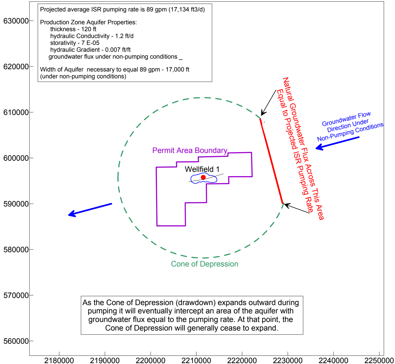
FIGURE OP-10 Conceptualization of the Limit of the Cone of Depression During ISR Operations
