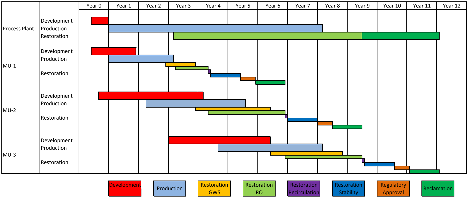
Figure RP-1 Lost Creek Project Development, Production and Restoration Schedule
