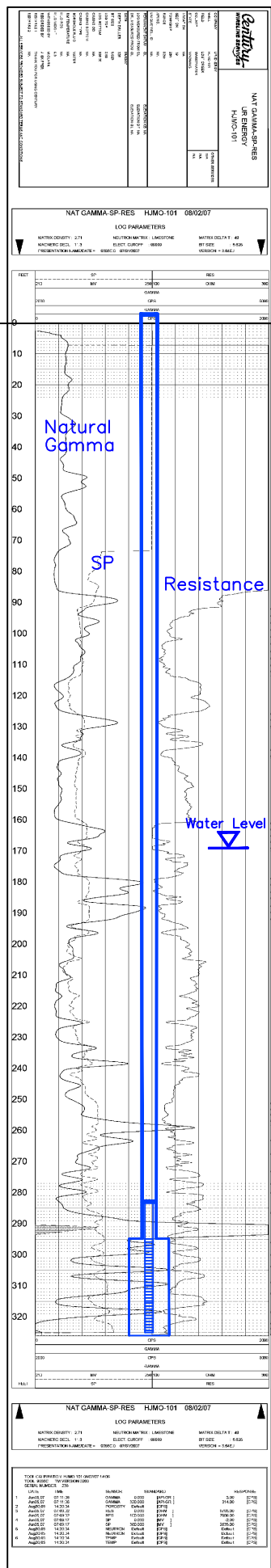
Vertical Scale: 1"=50'
