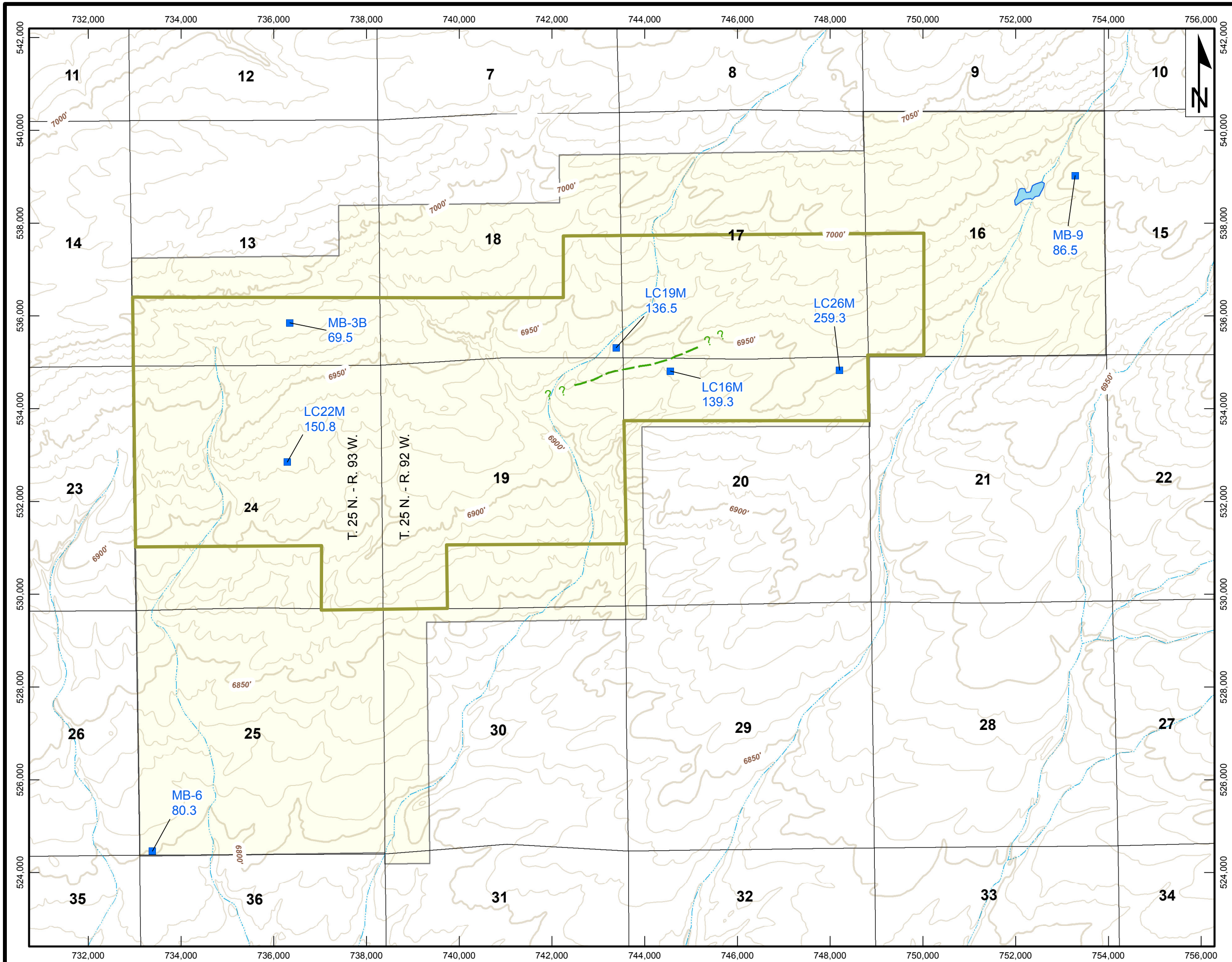
FIGURE V-8 Distribution of Average Sulfate September 2006 to July 2010
