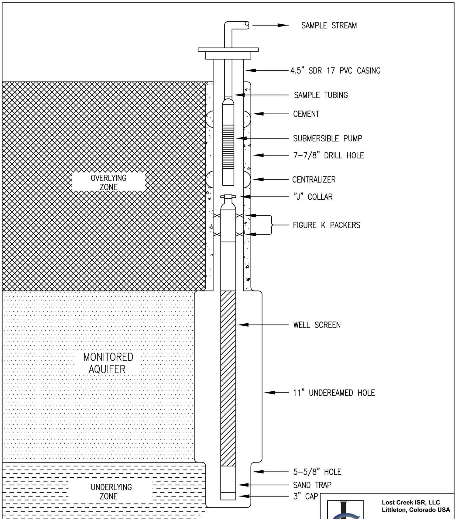
FIGURE VII-4 Monitor Well Construction Lost Creek Permit Area
