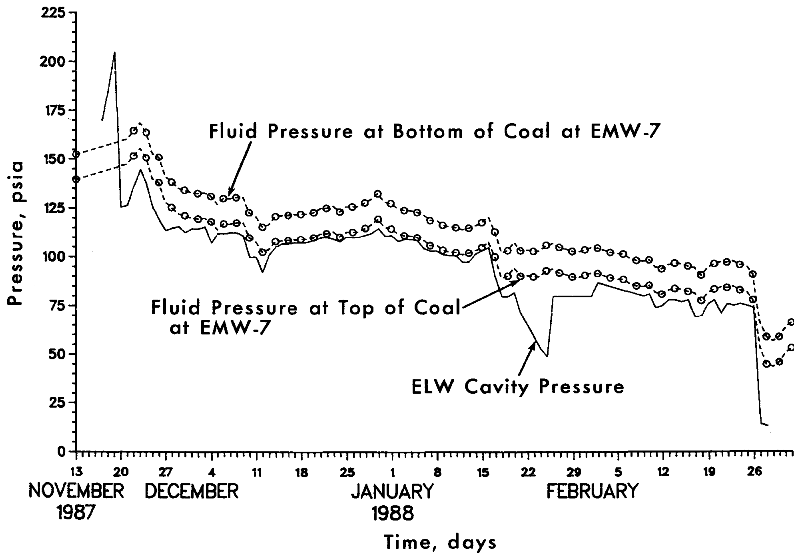
Figure 3-8. Fluid Pressure in the Coal Aquifer at EMW-7 Relative to ELW Cavity Pressure During the RM1 Test
