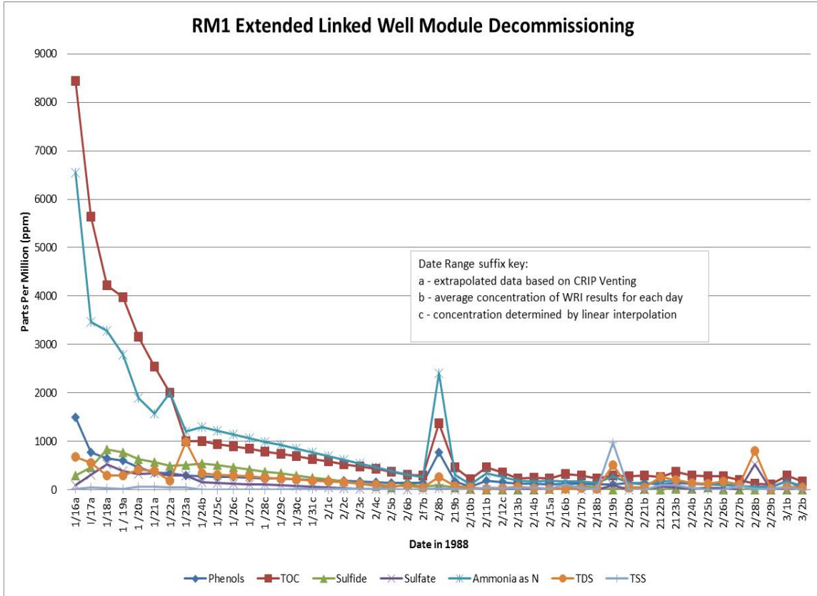
Figure 17-1: RM1 ELW Cavity Decommissioning and Restoration Contaminant Trends, Part 1
