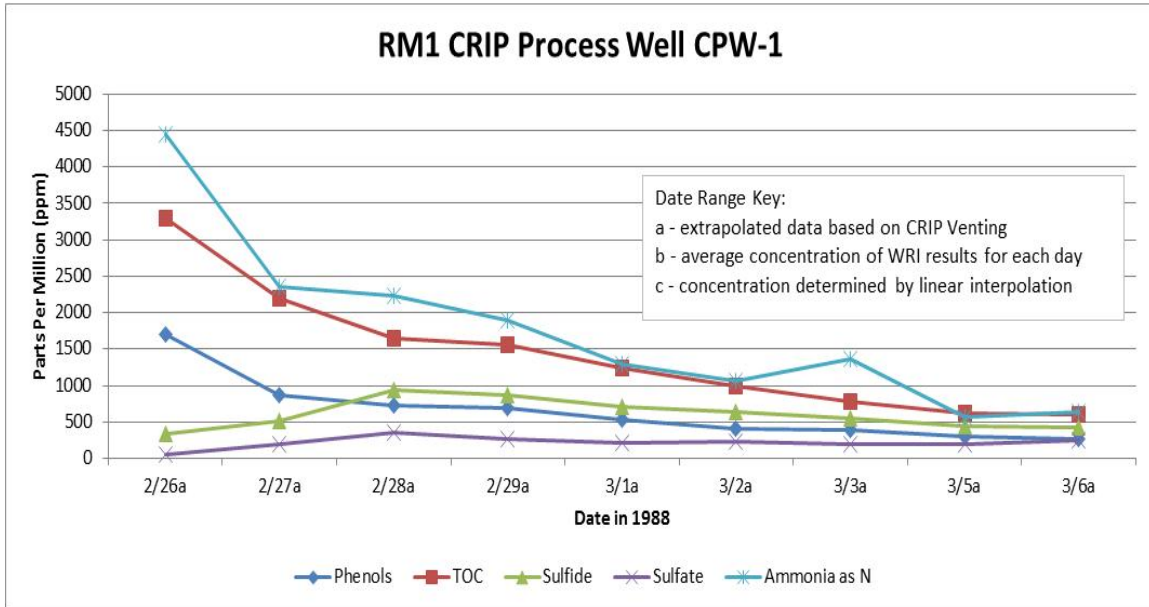
Figure 17-3: RM1 CRIP Cavity Decommissioning and Restoration Contaminant Trends, Part 1
