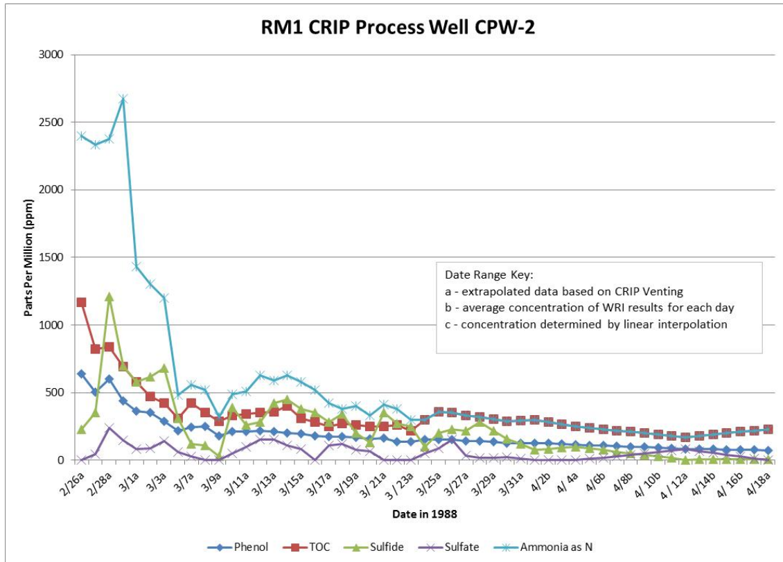
Figure 17-4: RM1 CRIP Cavity Decommissioning and Restoration Contaminant Trends, Part 2
