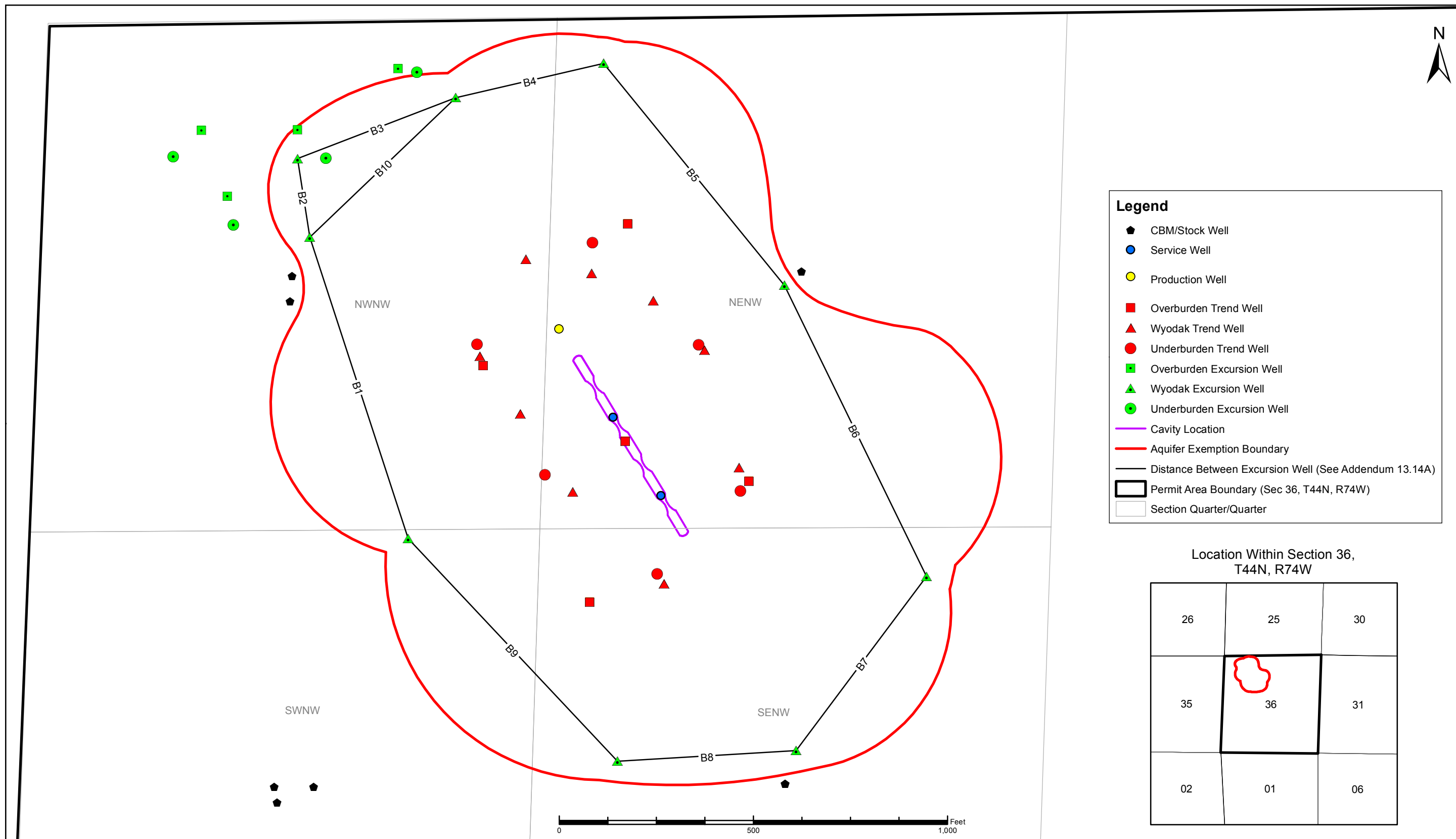
FIGURE 13.14-1: PROPOSED AQUIFER EXEMPTION AREA WITHIN NW 1/4, SEC 36, T44N, R74W
